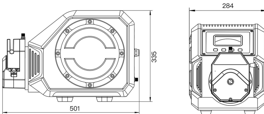
Dimension Drawing(mm)
